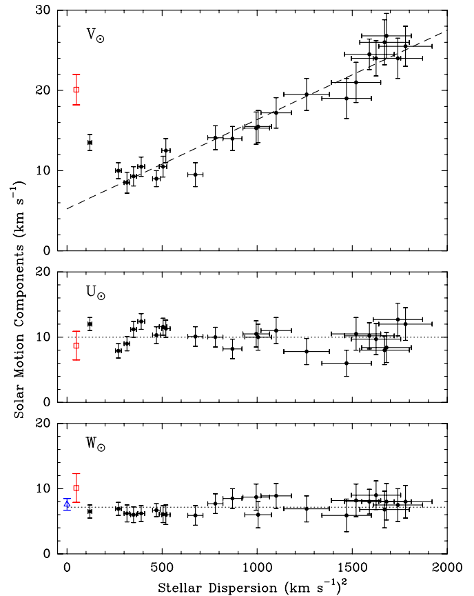
Figure 4. Solar motion components determined from Hipparcos stars (i.e., the reflex of the average motion of stars) vs. stellar velocity dispersion after Dehnen & Binney (1998). Top Panel: V_\odot is the Solar Motion in the direction of Galactic rotation (i.e., toward \ell = 90^\circ ). The “asymmetric drift” is shown with the dashed line. Middle Panel: U_\odot is the Solar Motion toward the Galactic center. Bottom Panel: W_\odot is toward the north Galactic pole. Also plotted at 50 (km s -1 ) 2 dispersion with open red squares are solar motion parameters obtained from the parallax and proper motions of star forming regions, and at zero dispersion with an open triangle is the W_\odot component inferred from the proper motion of Sgr A* by Reid & Brunthaler (2004). Note the good agreement of the U_\odot and W_\odot components between Hipparcos and this study. The large deviation of the V_\odot component from the asymmetric drift from this study is not indicative of large V_\odot value, but points to a significant deviation from circular orbits for very young stars.
