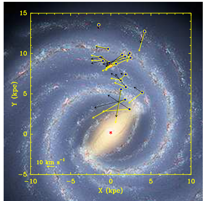
Figure 3. Peculiar motion vectors of HMSFRs (superposed on an artist conception) projected on the Galactic plane after transforming to a reference frame rotating with the Galaxy. A 10 \text{ km s}^{-1} motion scale is in the lower left. The Galaxy is viewed from the north Galactic pole and rotates clockwise. The light (yellow) arrows are for IAU standard values of R_0 = 8.5 \text{ kpc} and \Theta_0 = 220 \text{ km s}^{-1} and a flat rotation curve, whereas black arrows are for \Theta_0 = 254 \text{ km s}^{-1} . This demonstrates that the qualitative result that HMSFRs orbit the Galaxy slower than the Galaxy rotates is not sensitive to the value of \Theta_0 .
