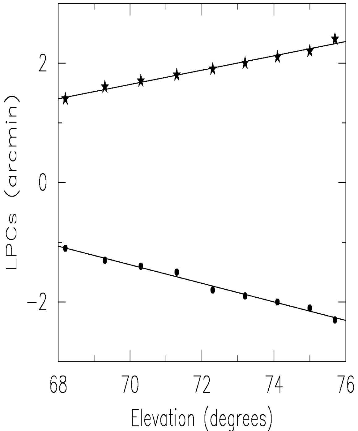
Figure 1: The local pointing corrections (LPCs) are determined from cross scans made on 3C147 as a function of elevation. The nominal LPCs ( \Delta Az_2 = 5'.6 , \Delta El = 4'.8 ) are used and not updated after each cross scan. The filled circles are \Delta Az_2 and the filled stars \Delta El . A least-squares linear fit is made to each LPC. \Delta Az_2 is changing 0'.15 per degree in elevation, while \Delta El is changing 0'.12 per degree in elevation. The fits is good to within \sim 5\% .
